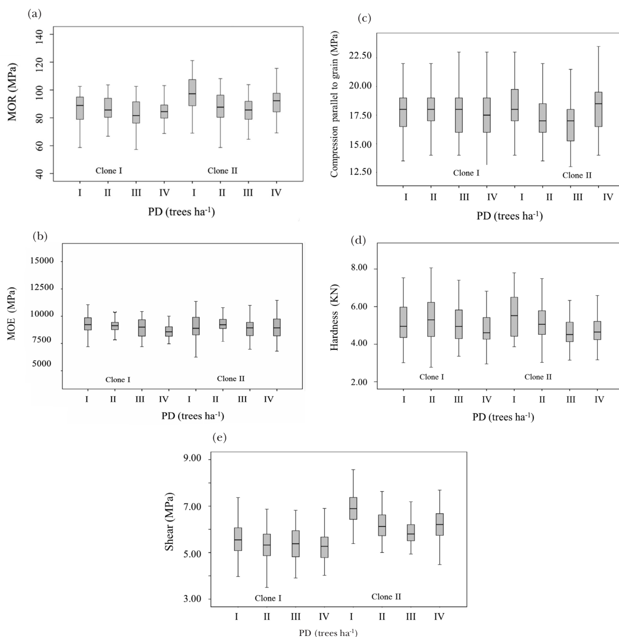
Figure 2 Box-plots of (a) MOR, (b) MOE, (c) compression, (d) hardness and (e) shear parallel to grain measured at different planting densities of the two clones; a box represents the interquartile range; a line across the box indicates the mean; bars extend from the box to the highest and lowest values; MOR = modulus of rupture; MOE = modulus of elasticity; PD = planting density
