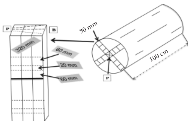
Figure 1 Schematic diagram of the samples prepared for mechanical property determination; P = pith, B = bark
